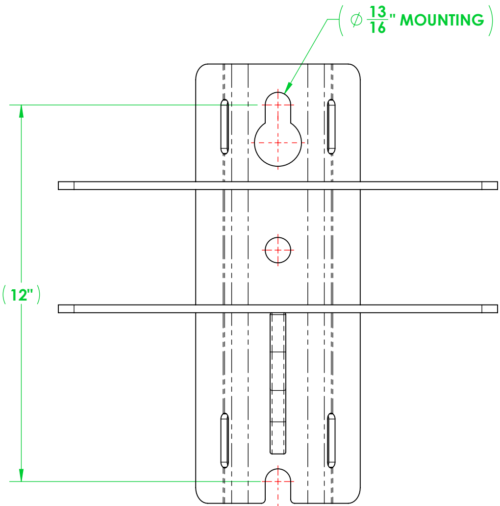
DETAIL A
